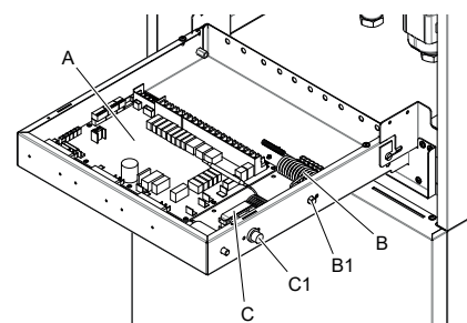
fig. 12 - internal view of the electric box
