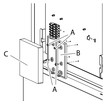
fig. 18 - Installation of the remote control
